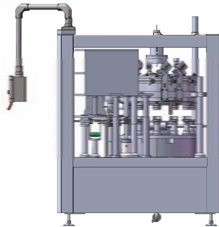
CRAFTBLOC 12/1-45 CPM FILLER/SEAMER
